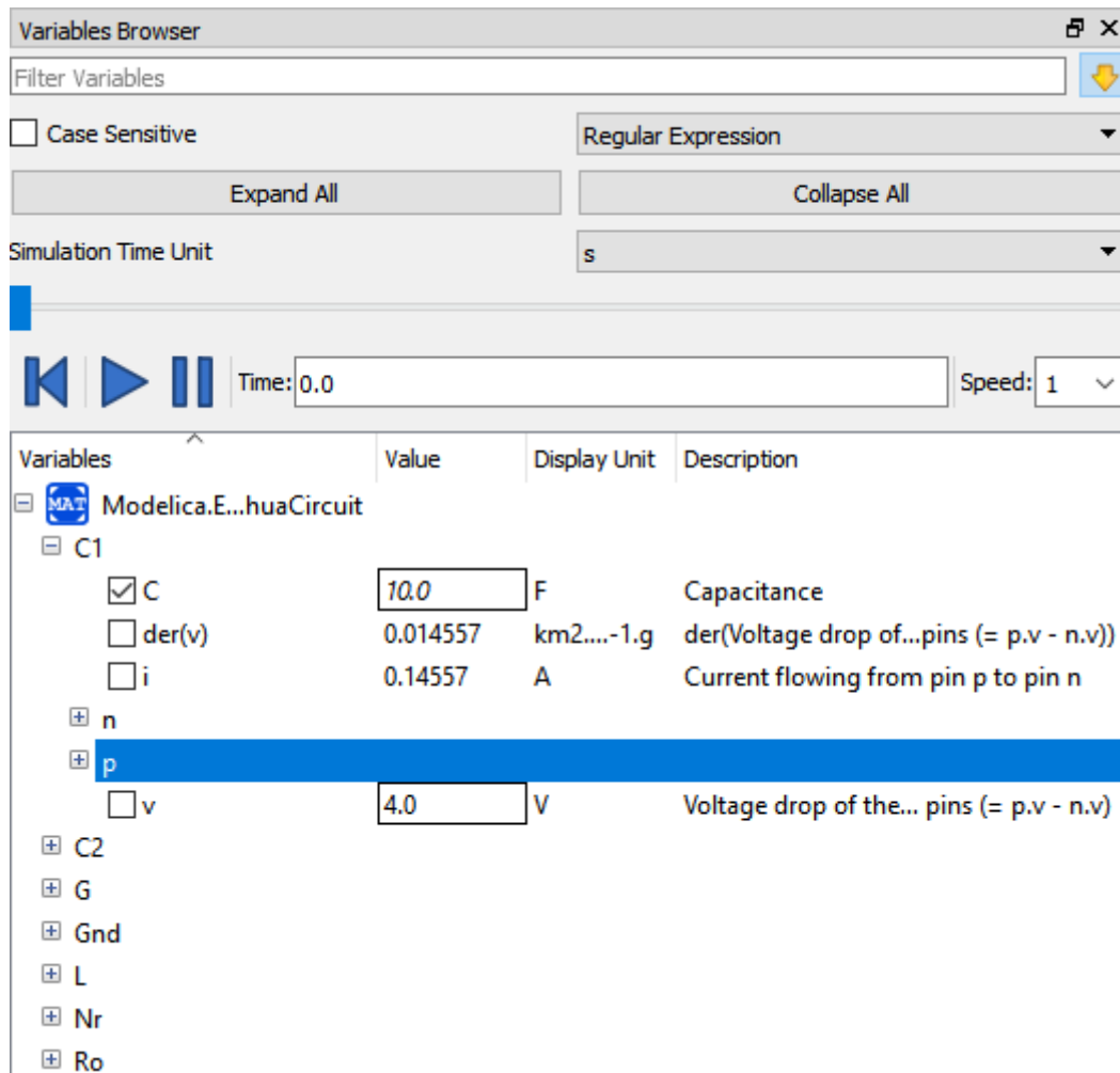
Figure 2.5: Variables Browser.
