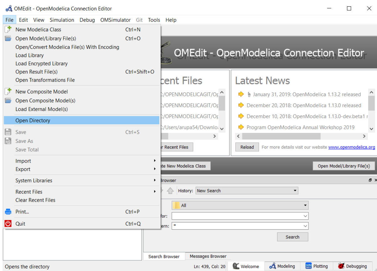
Figure 2.16: open-directory
