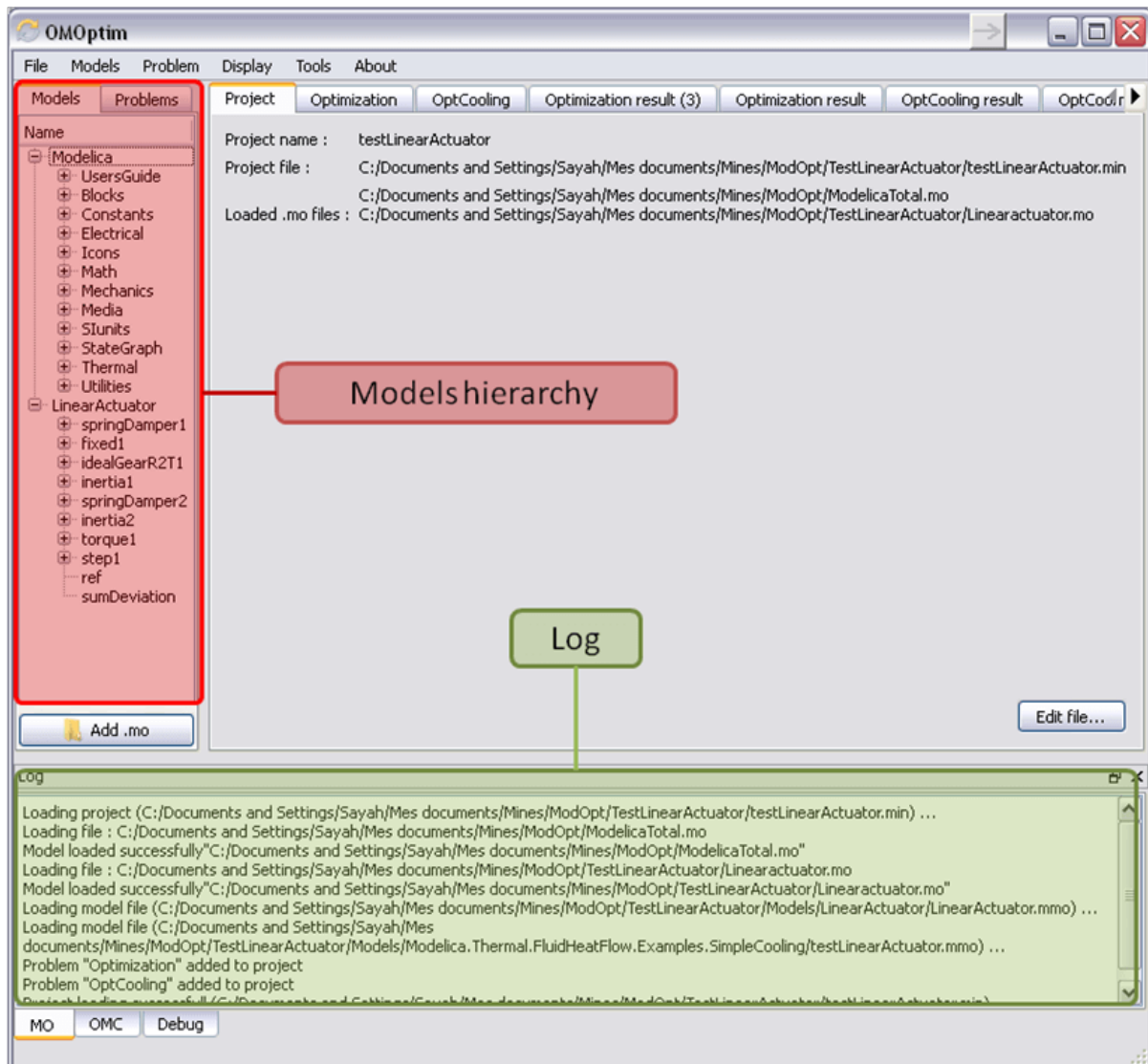
Figure 11.3: OMOptim window after having loaded model.
