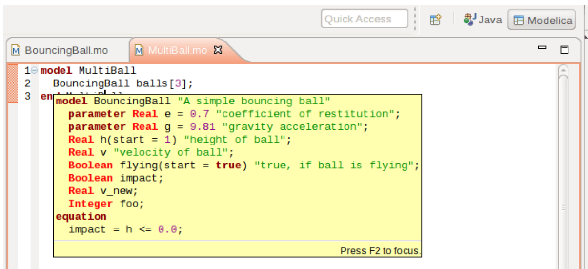
Figure 14.13: Displaying information for identifiers on hovering.
