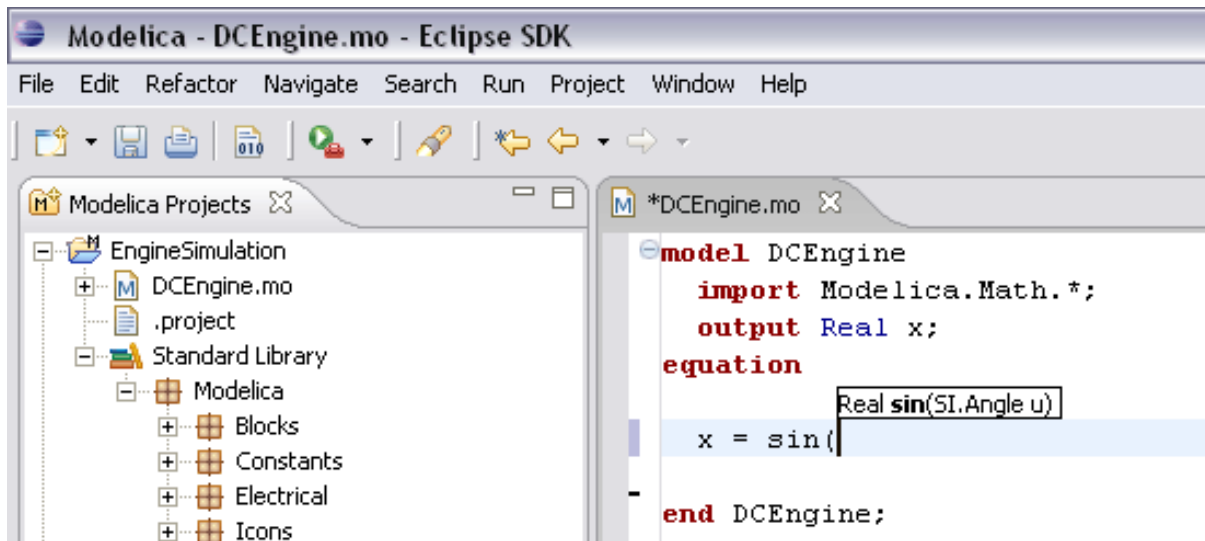
Figure 14.12: Code completion at a function call when typing left parenthesis.
