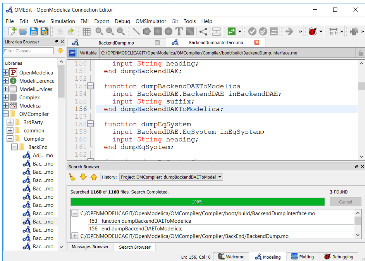
Figure 2.20: Search Results
