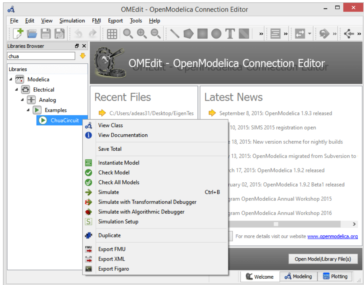
Figure 2.3: Libraries Browser.
