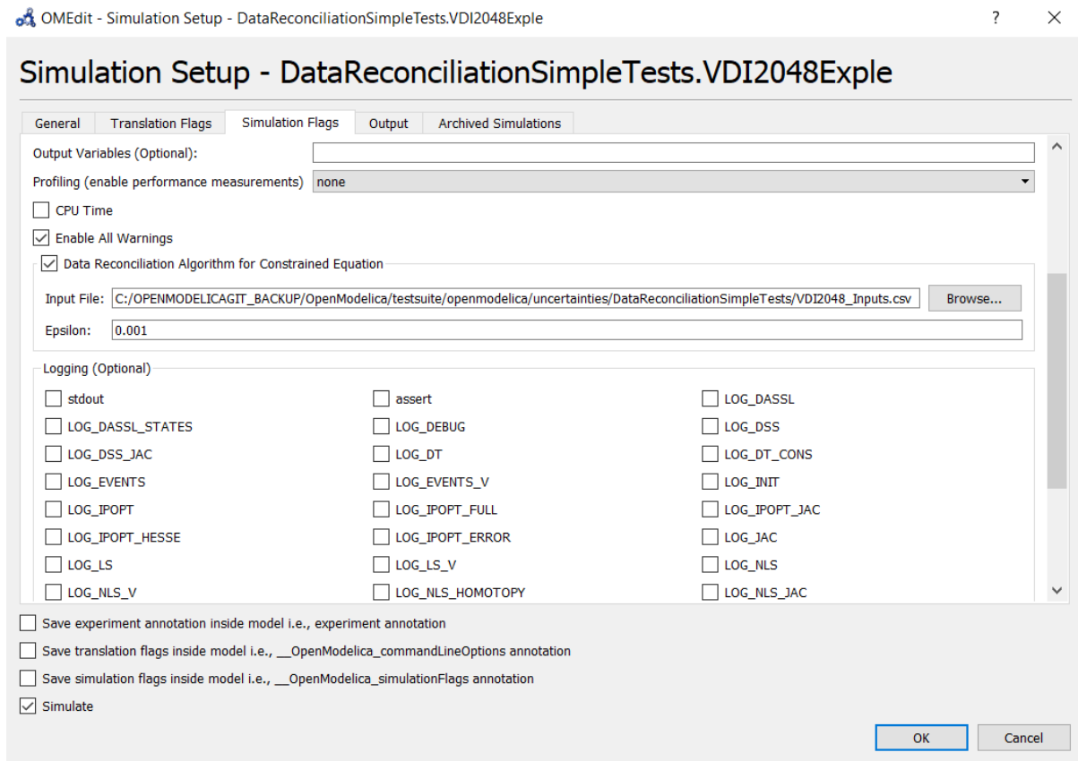
Figure 27.3: Setting DataReconciliation SimulationFlag
