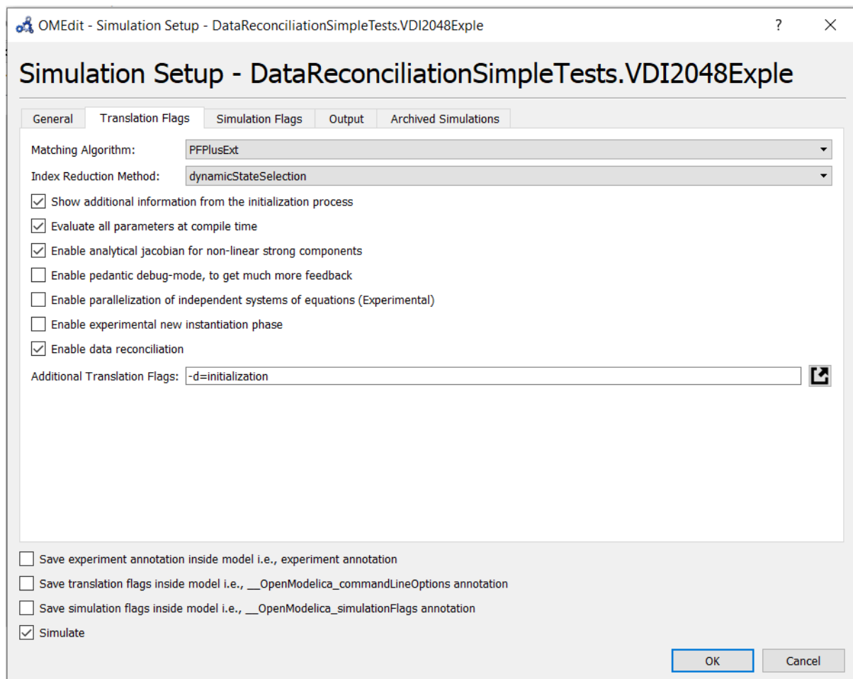
Figure 27.2: Setting DataReconciliation TranslationFlag
