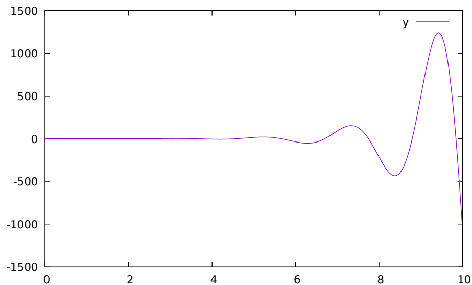
Figure 10.12: Characteristic equation with imaginary roots with positive real part.
