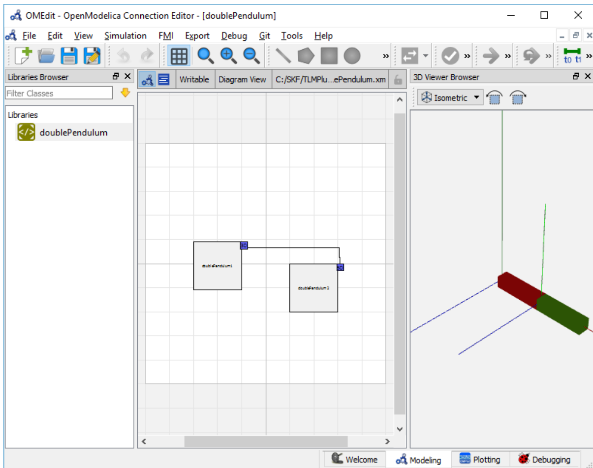
Figure 7.2: Composite Model with 3D View.
