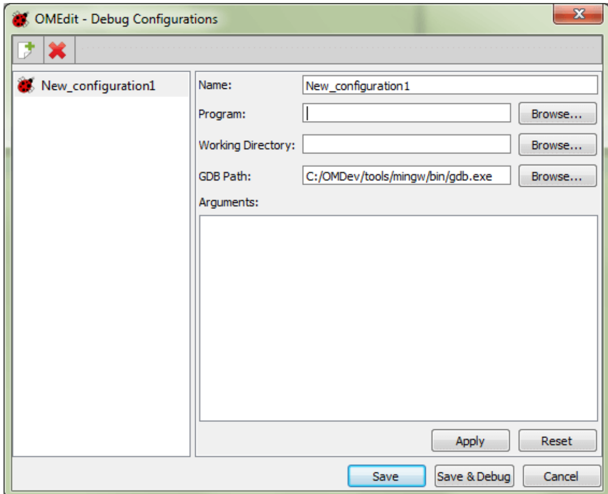
Figure 5.4: Debug Configurations.
