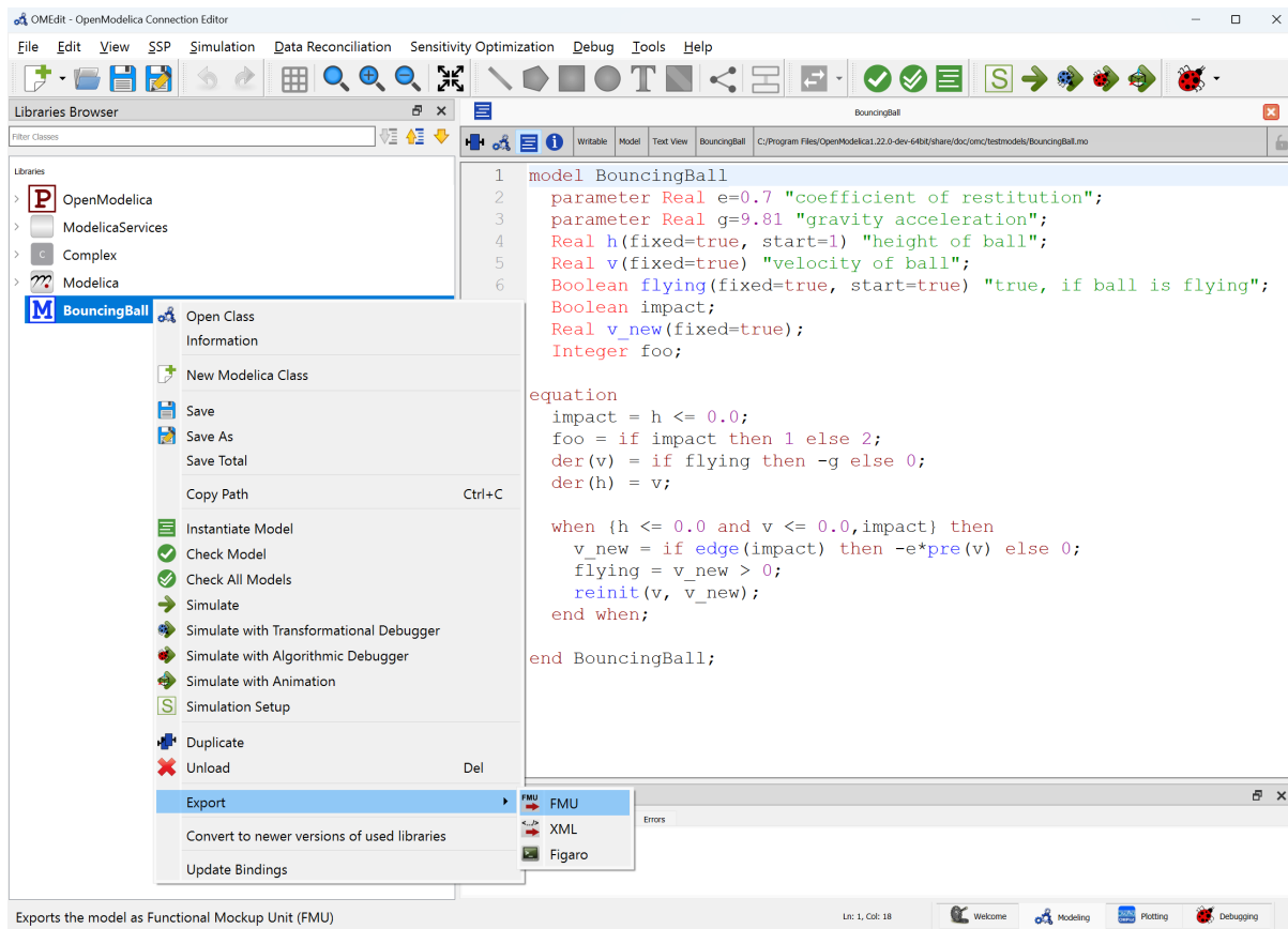
Figure 11.1: FMI Export.
