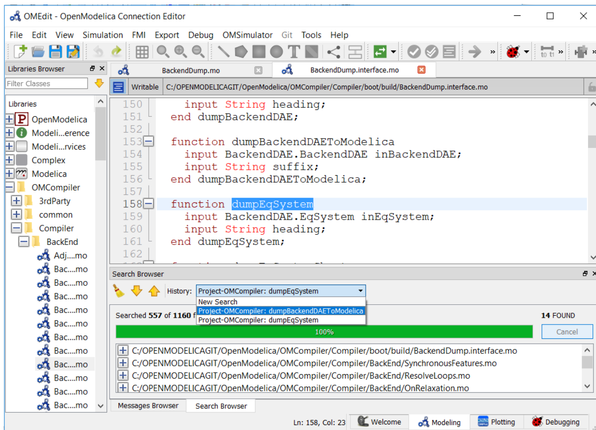
Figure 3.23: Search History
