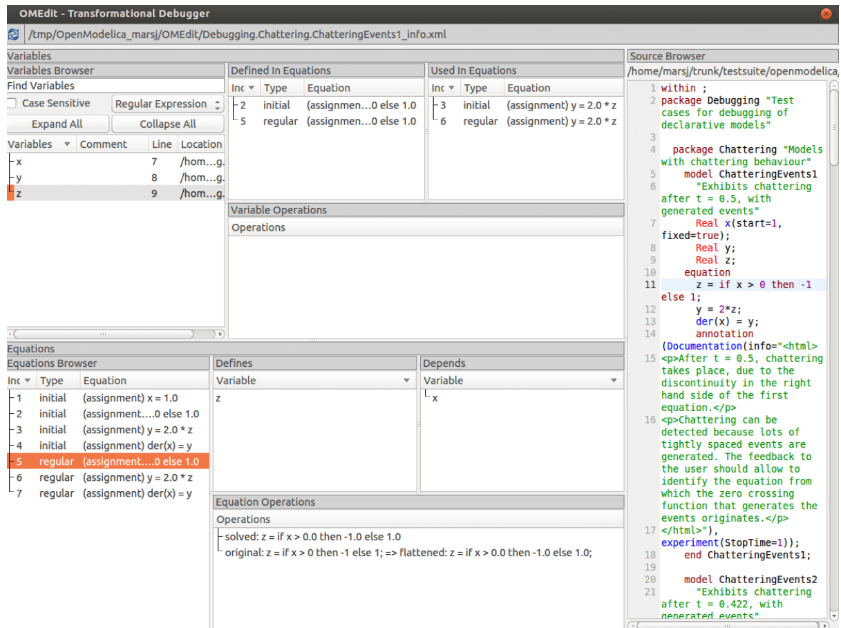
Figure 7.2: Transformations Browser.
