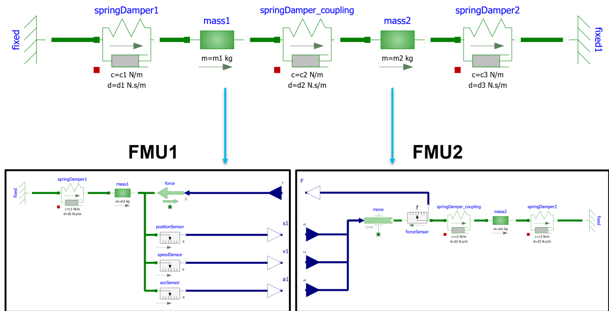
Figure 13.11: Dual mass oscillator Modelica model (diagramm view) and FMUs
