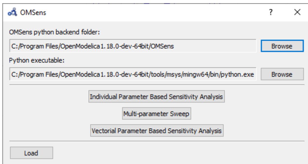
Figure 18.3: OMSens window.
