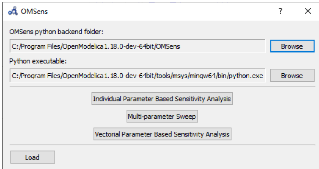
Figure 14.3: OMSens window.
