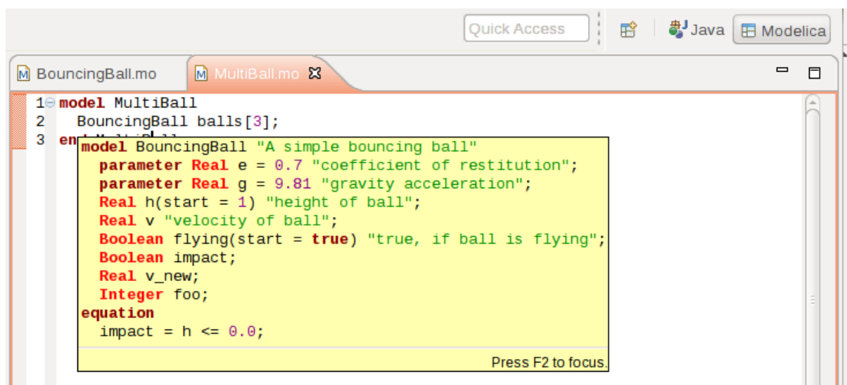
Figure 16.13: Displaying information for identifiers on hovering.
