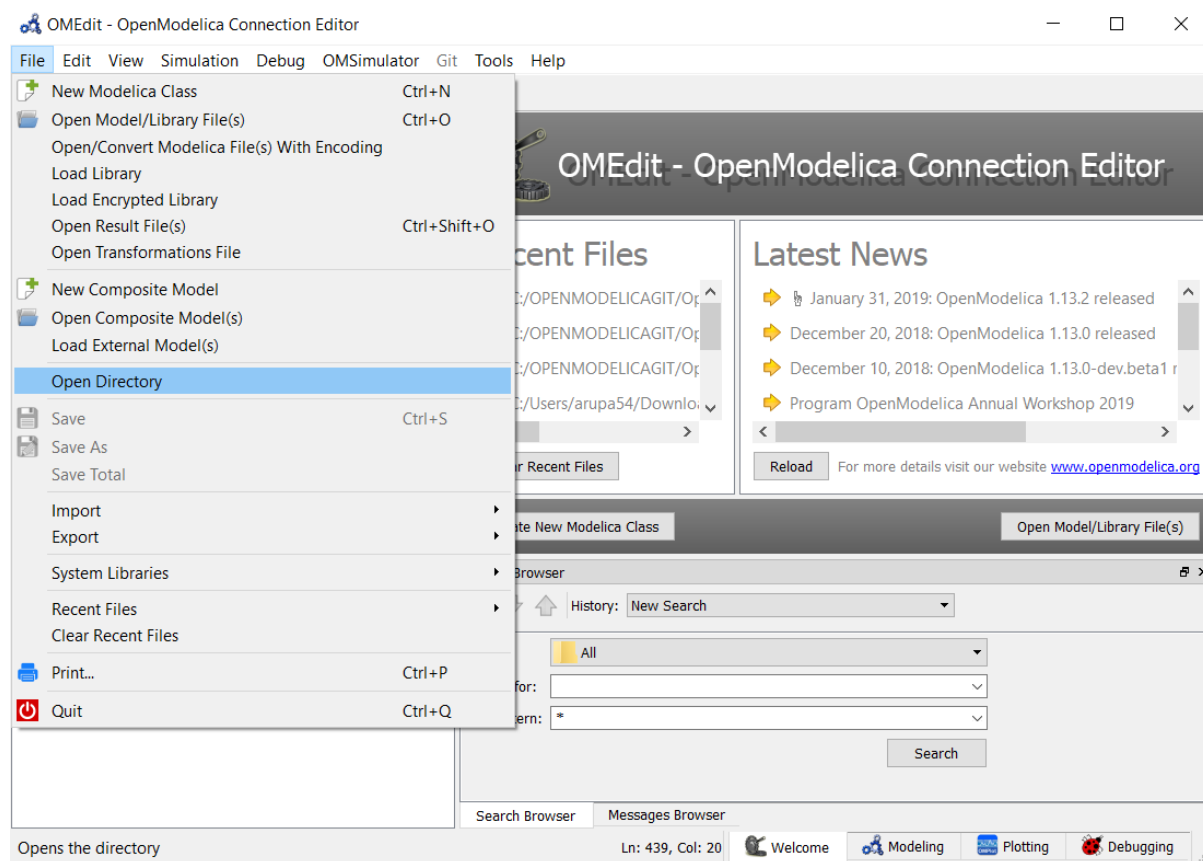
Figure 2.16: open-directory
