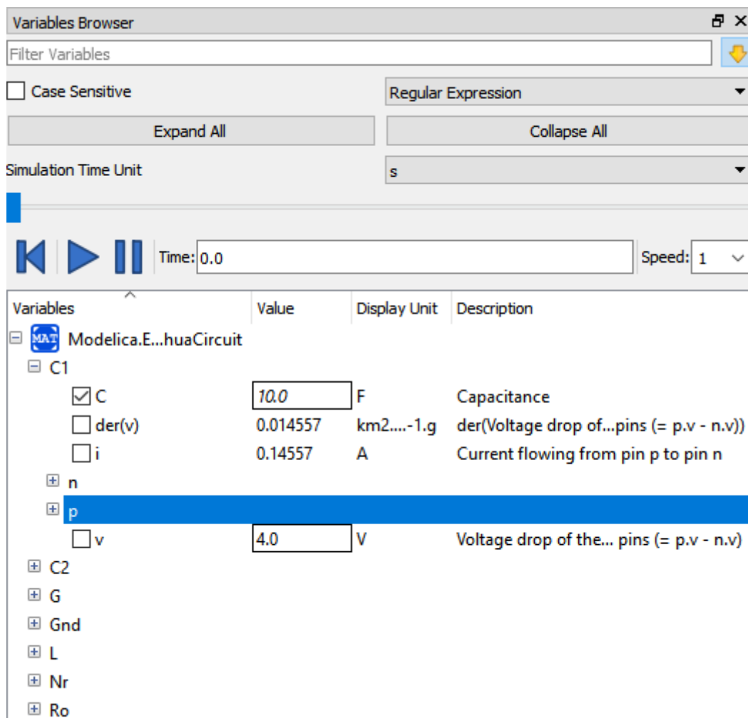
Figure 2.4: Variables Browser.
