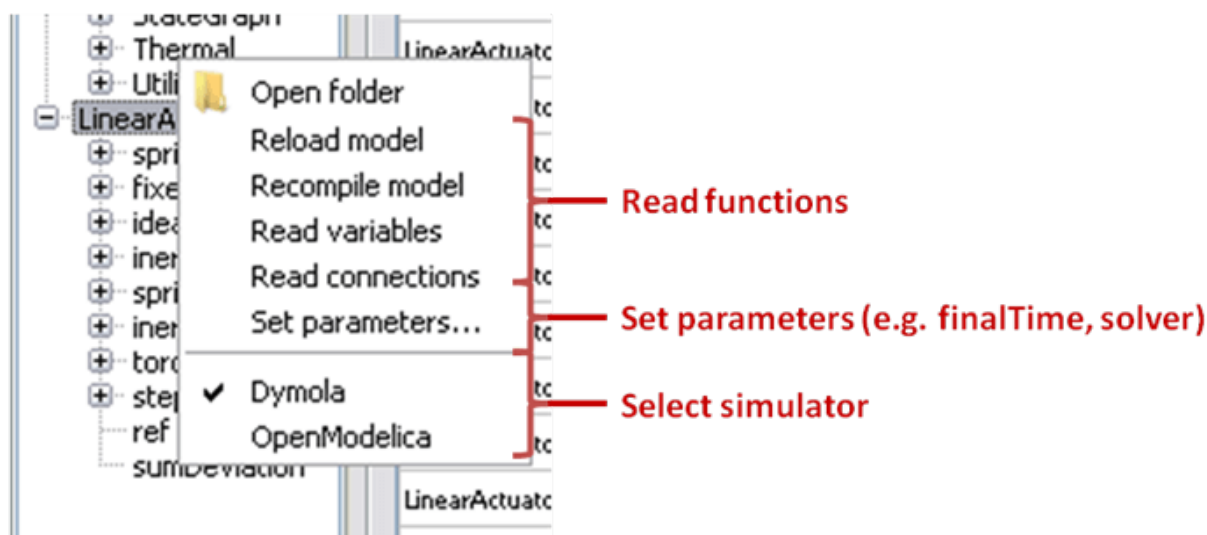
Figure 13.5: Selecting read variables, set parameters, and selecting simulator.
