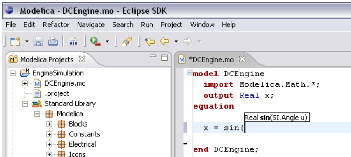
Figure 16.12: Code completion at a function call when typing left parenthesis.
