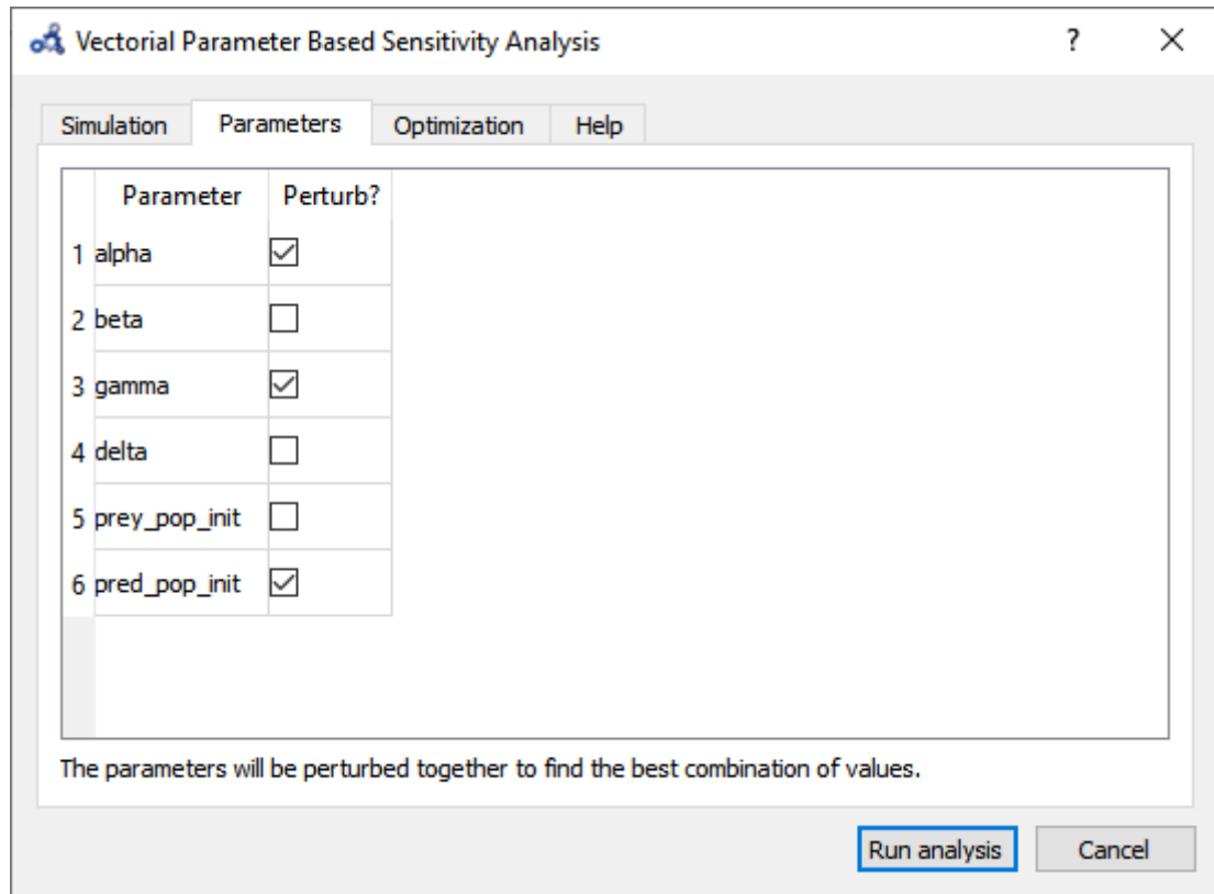
Figure 14.13: Vectorial sensitivity analysis parameters.
