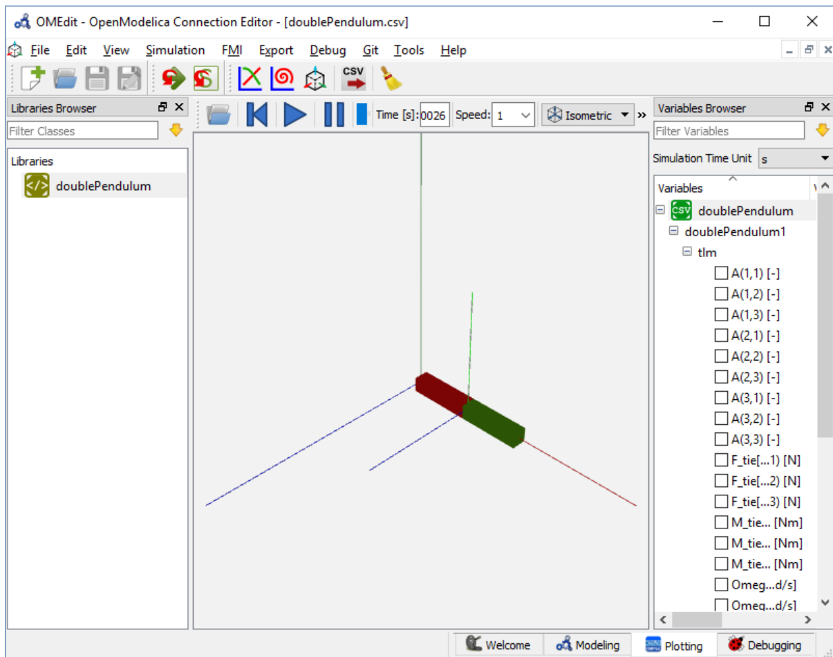
Figure 8.6: TLM Co-Simulation Visualization.
