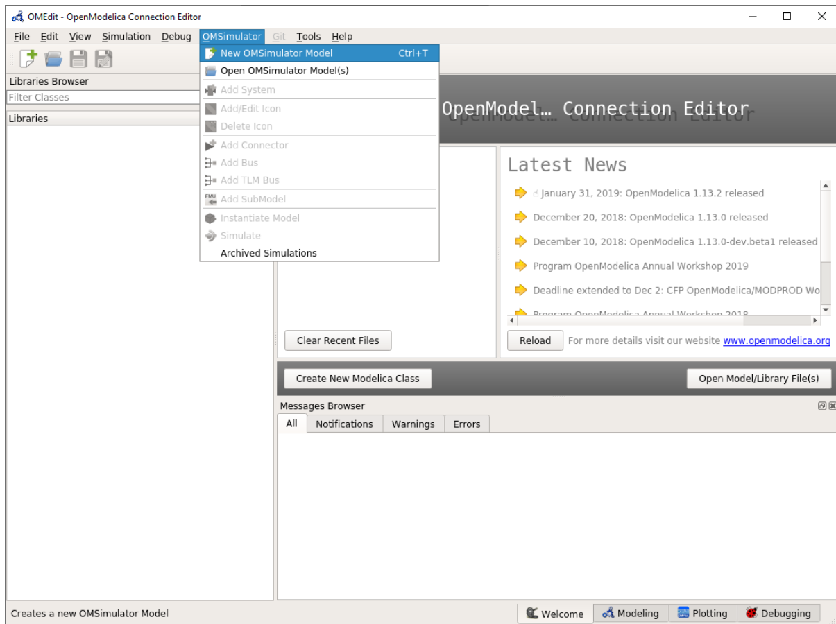
Figure 9.3: OMEdit: New OMSimulator Model
