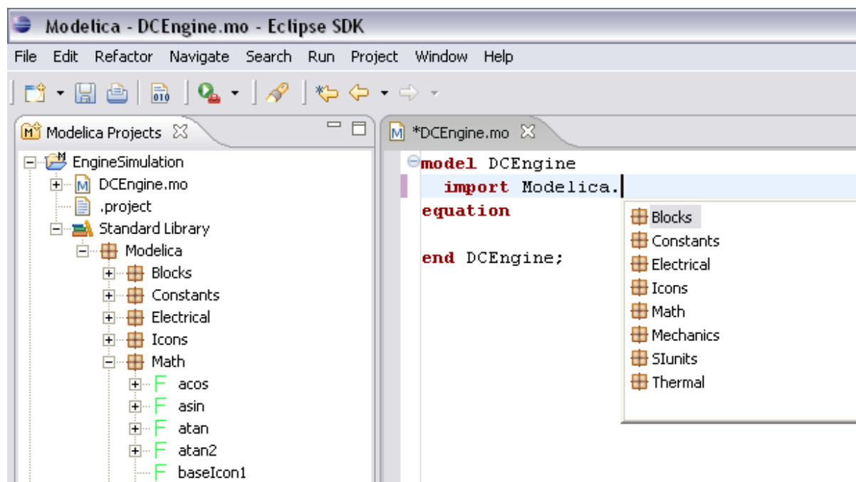
Figure 16.11: Code completion when typing a dot.
