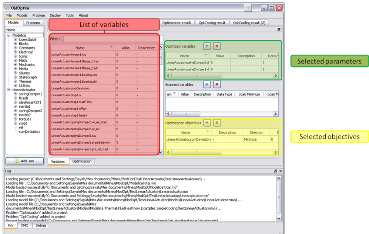
Figure 13.4: Forms for defining a new optimization problem.
