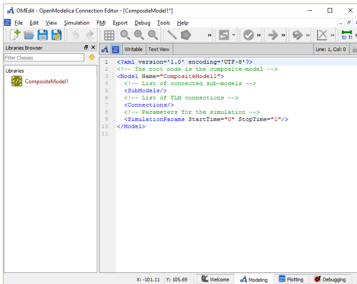
Figure 8.8: New composite model text view.
