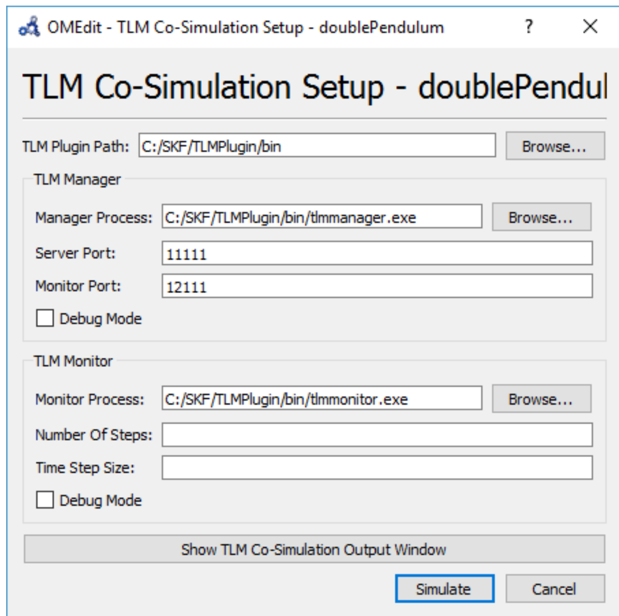
Figure 8.3: TLM Co-simulation Setup.
