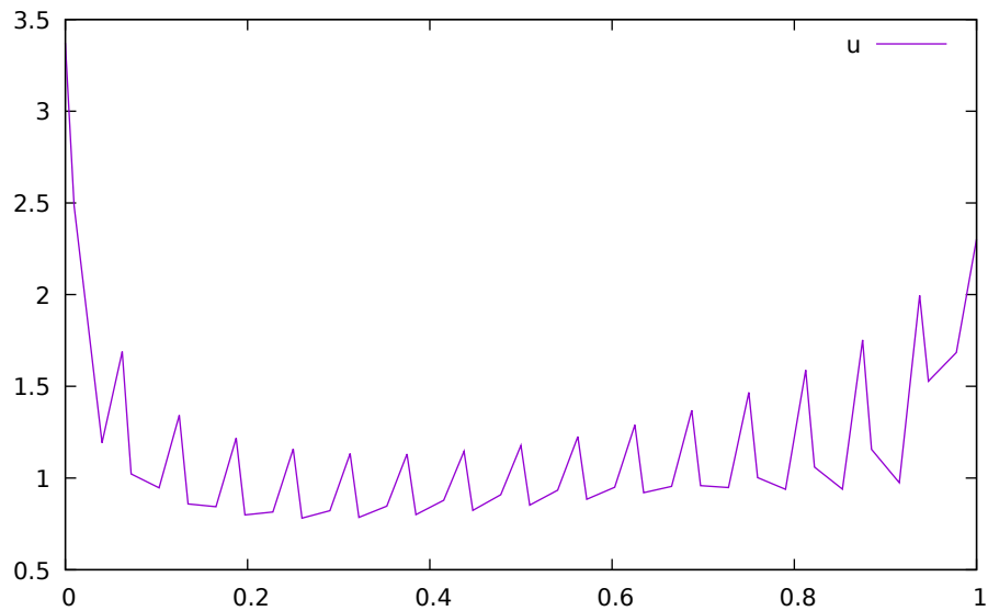
Figure 13.1: Optimization results for Batch Reactor model – input variables.
