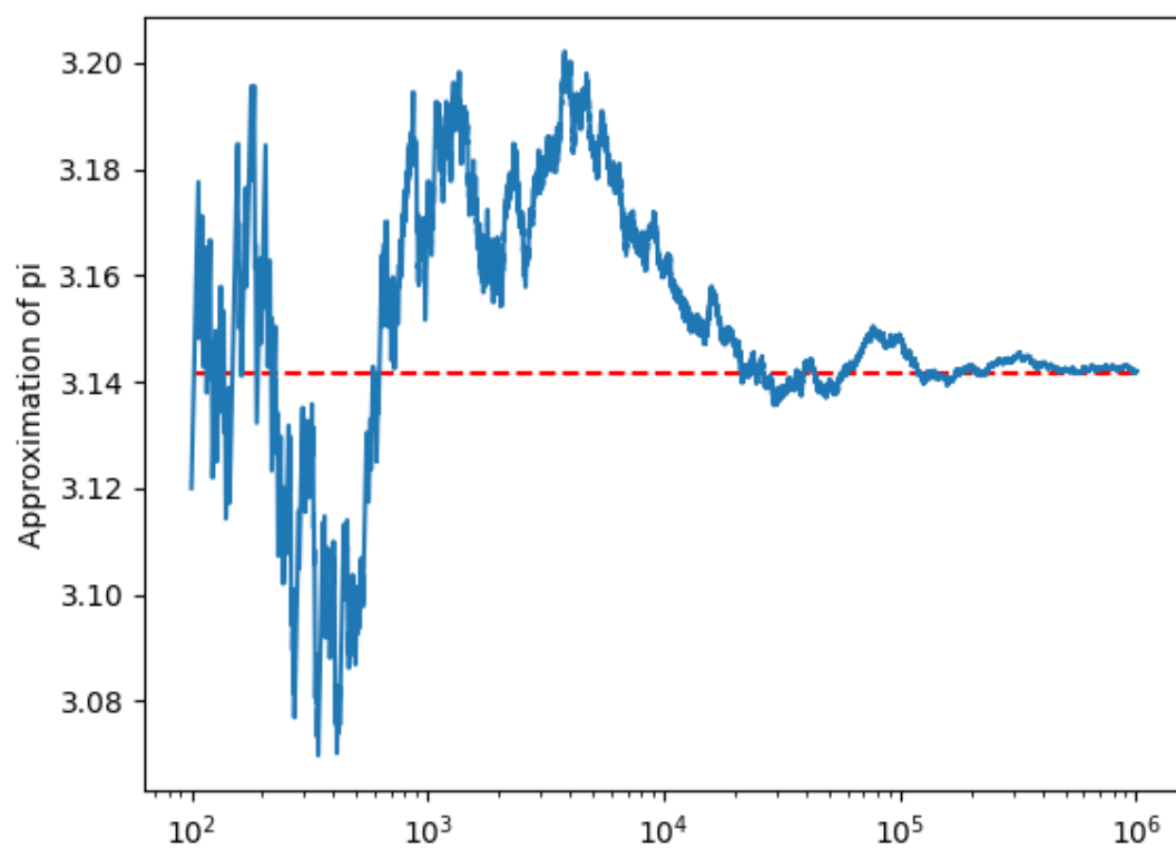
Figure 9.1: Results of the above batch simulation which approximates the value of pi
