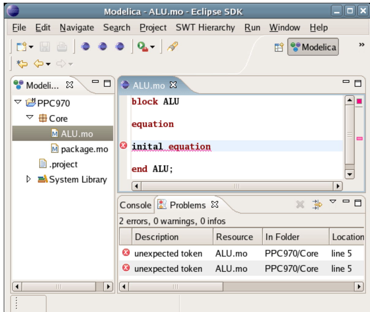
Figure 16.10: Syntax checking.
