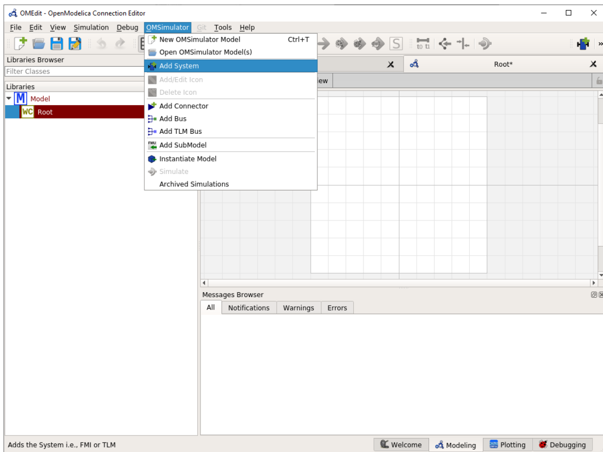
Figure 9.5: OMEdit: Add System
