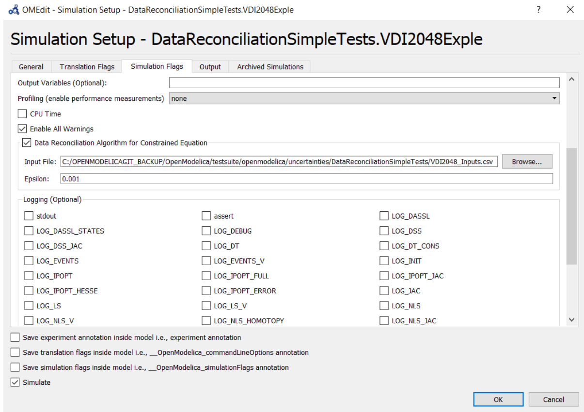
Figure 30.3: Setting DataReconciliation SimulationFlag
