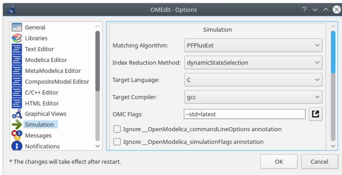
Figure 2.14: Ensure (at least) Modelica v3.3 support.
