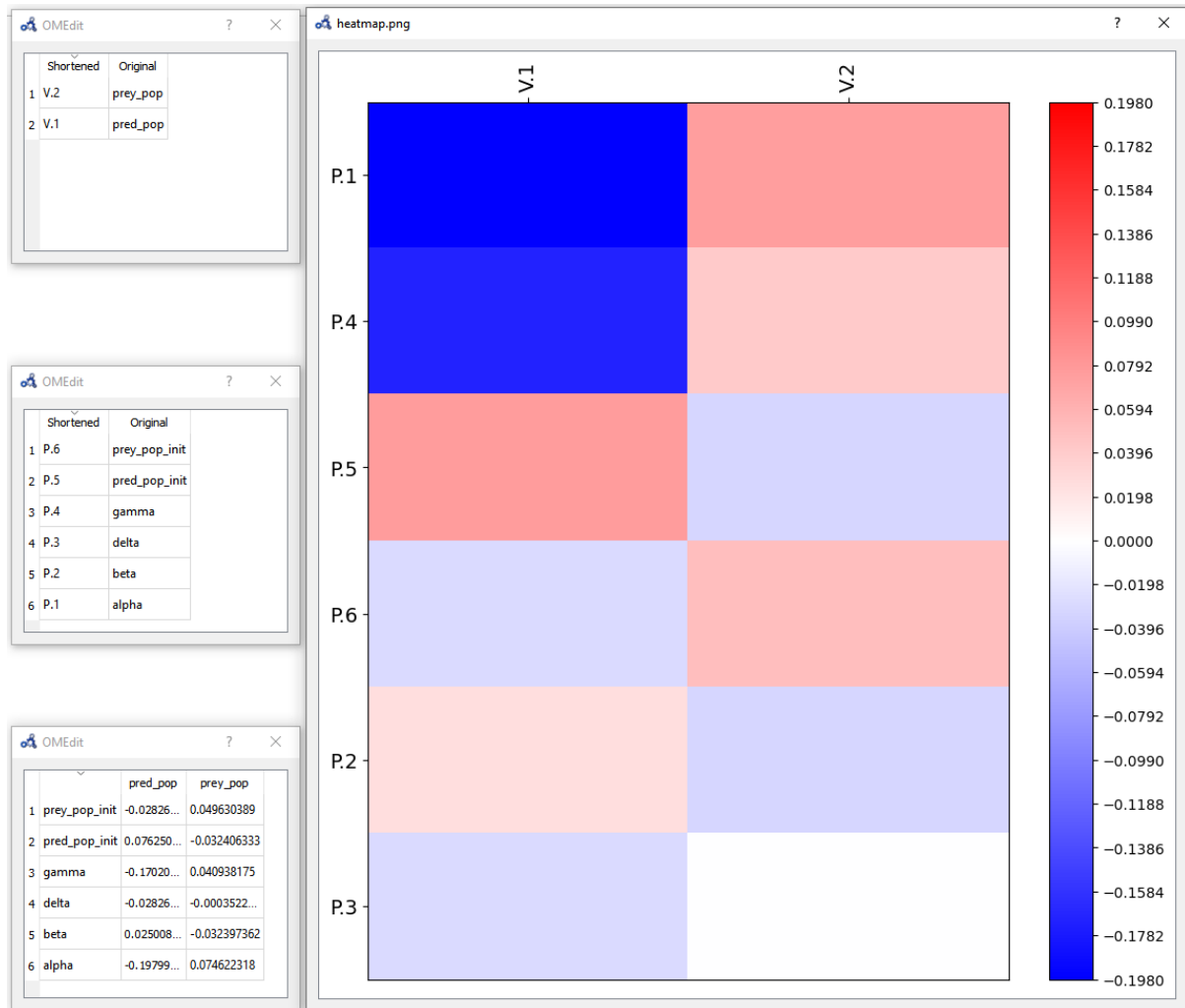
Figure 14.9: Individual sensitivity analysis heatmap.
