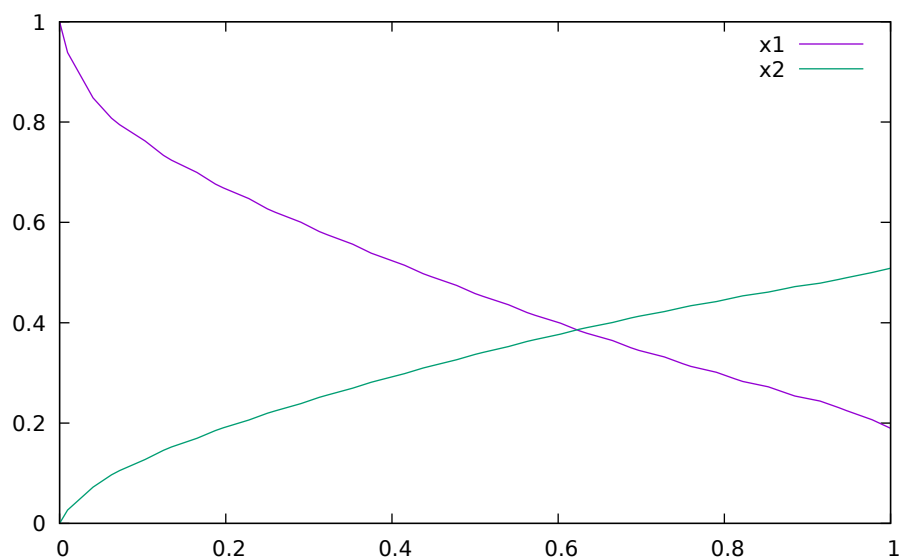
Figure 13.2: Optimization results for Batch Reactor model – state variables.
