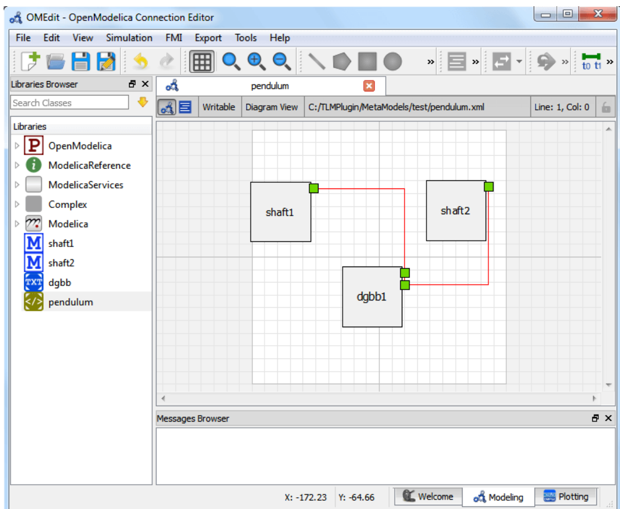
Figure 8.13: Connecting sub-models of the Double Pendulum Composite Model.
