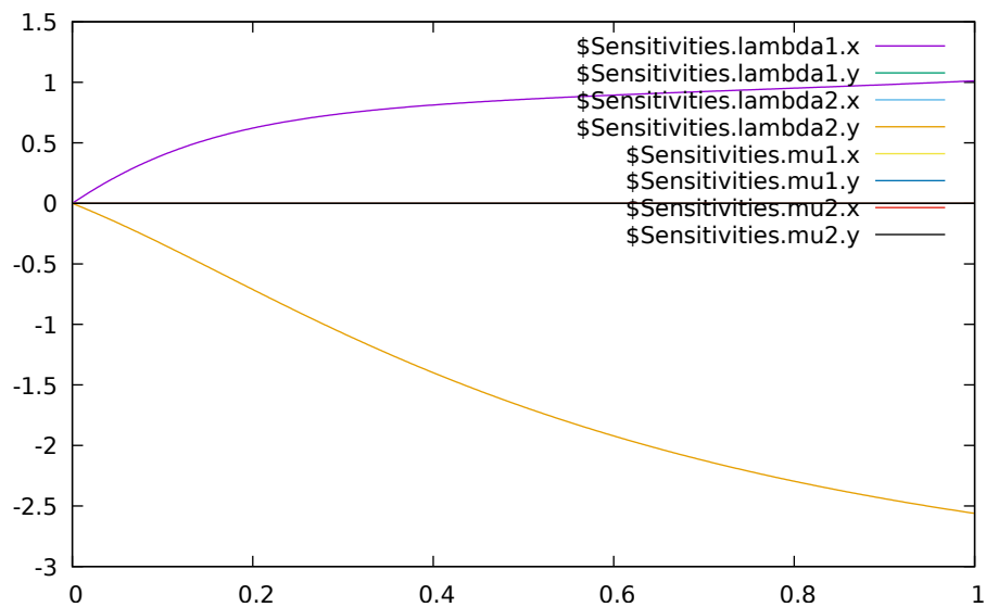
Figure 14.1: Results of the sensitivities calculated by IDA solver.
