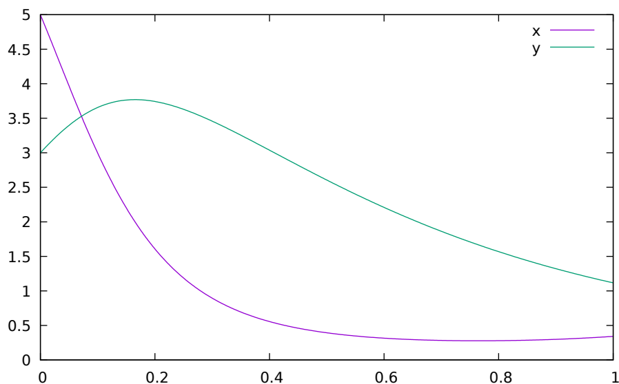
Figure 14.2: Results of the Lotka-Volterra equations.
