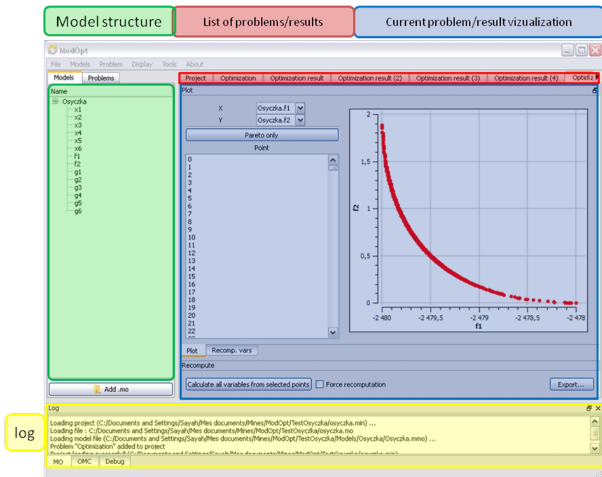
Figure 13.6: Window regions in OMOptim GUI.
