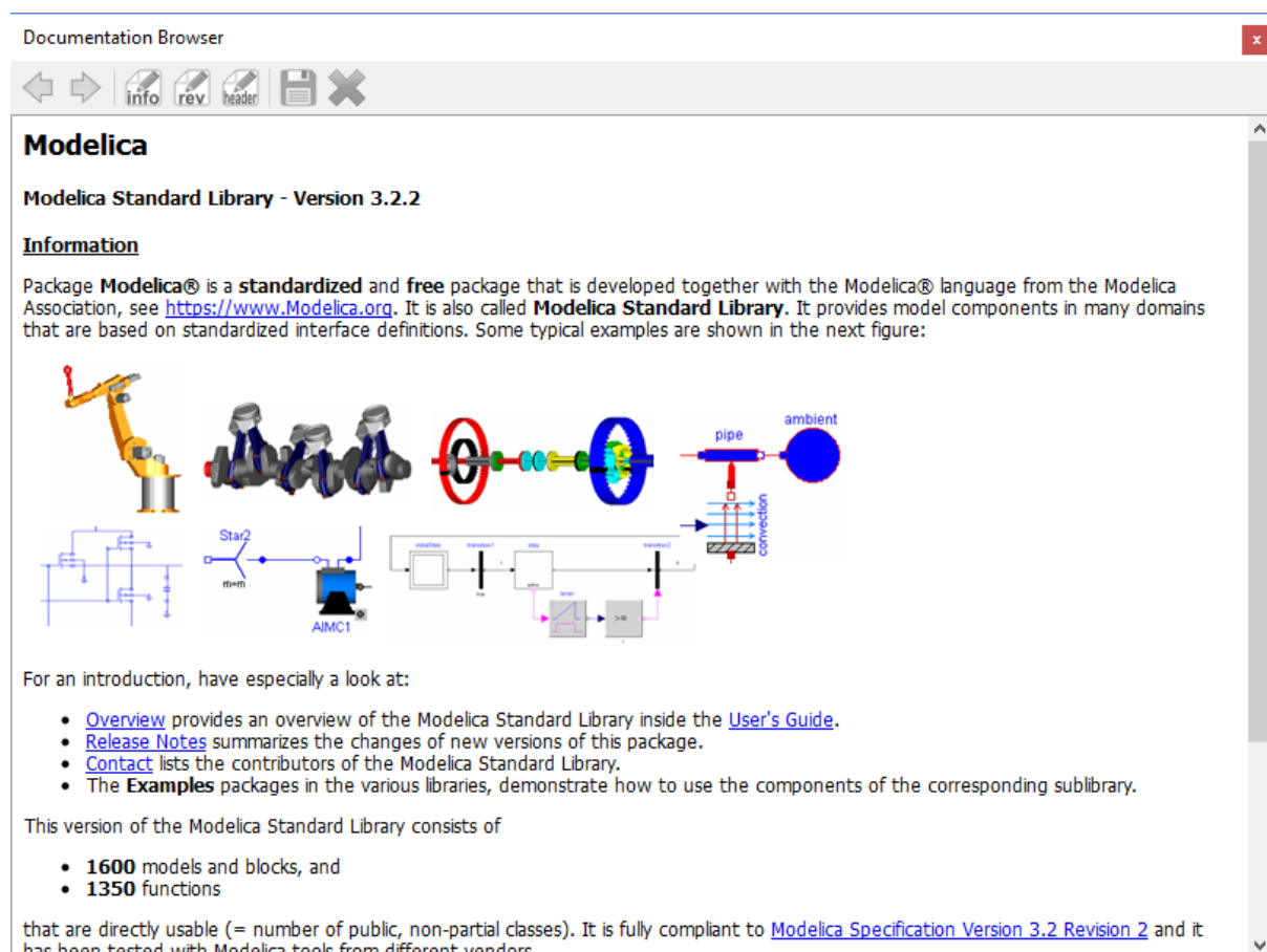
Figure 2.3: Documentation Browser.
