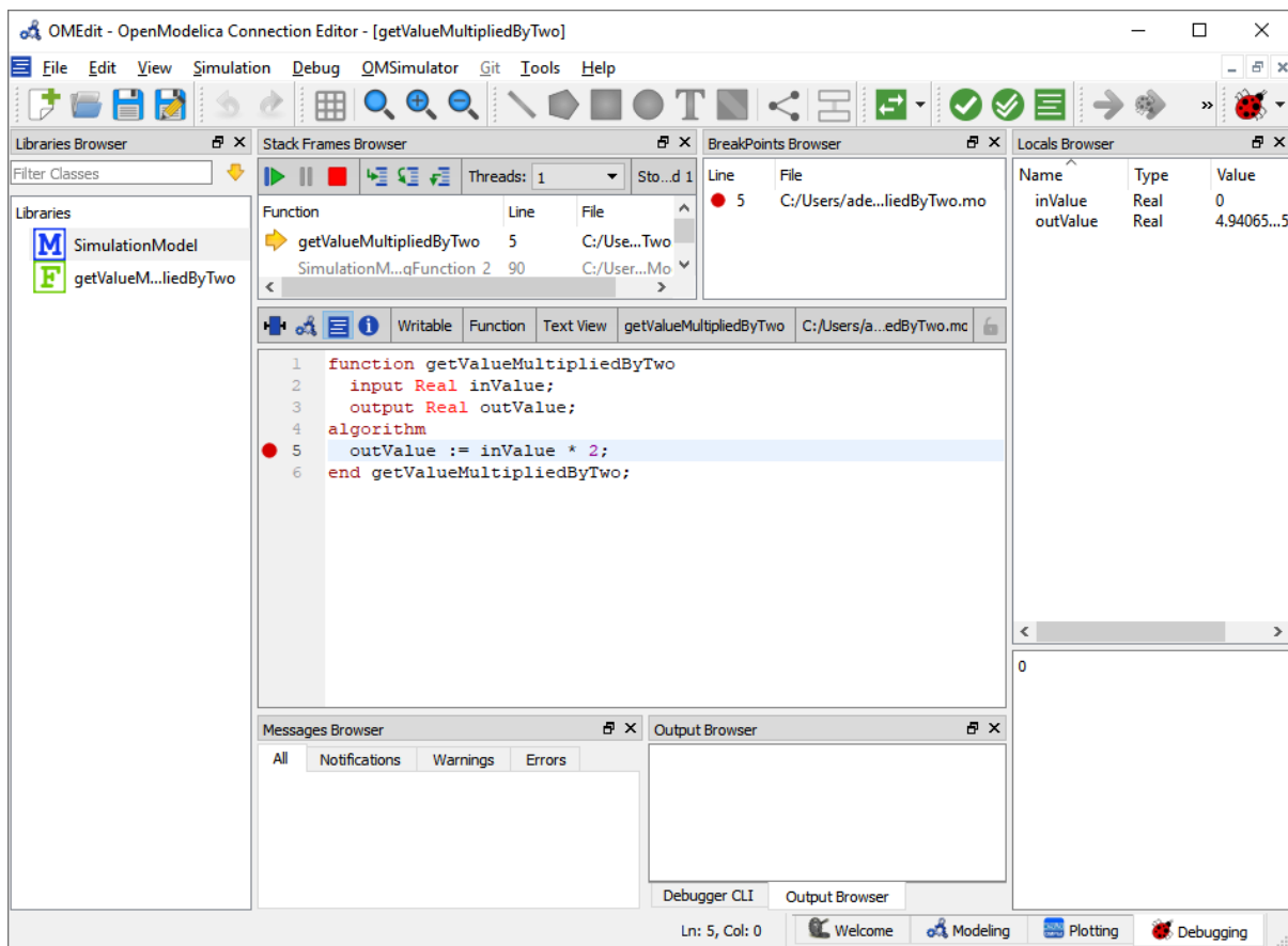
Figure 5.6: Algorithmic Debugger.
