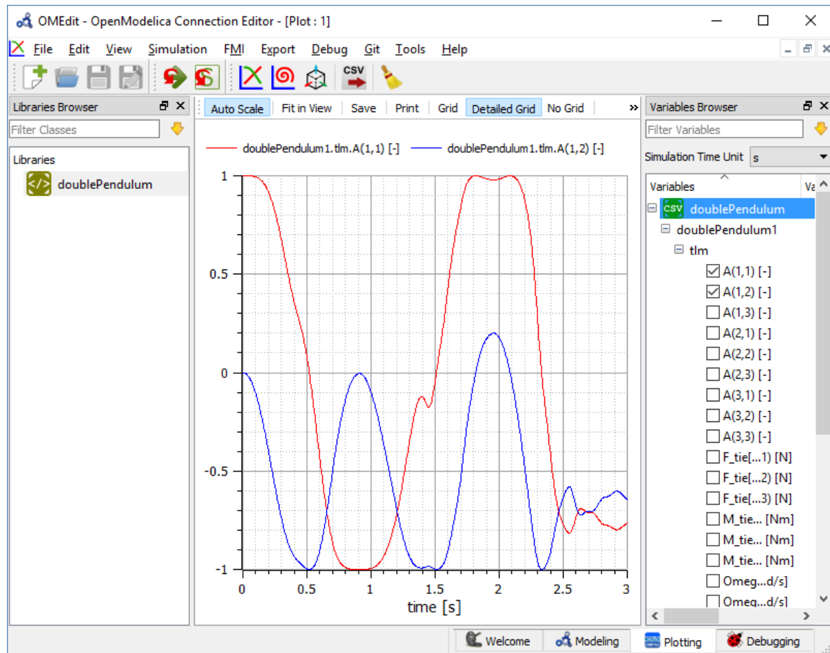
Figure 8.5: TLM Co-Simulation Results Plotting.
