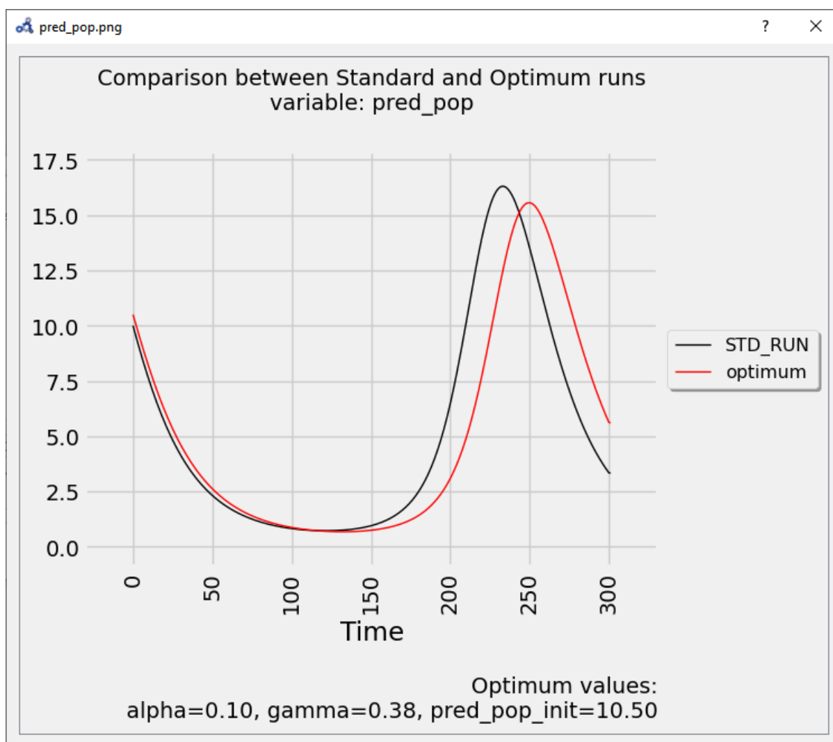
Figure 14.17: Vectorial sensitivity analysis plot.
